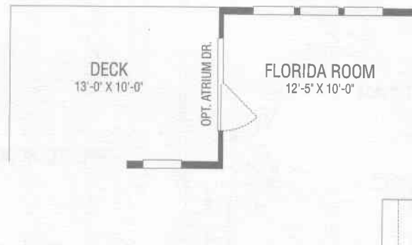
Partial First Floor Plan
